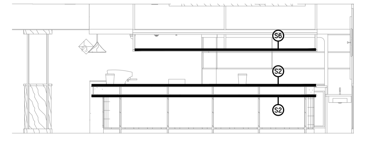
DETAIL C COCKTAIL BAR ELEVATION SCALE 1:50
